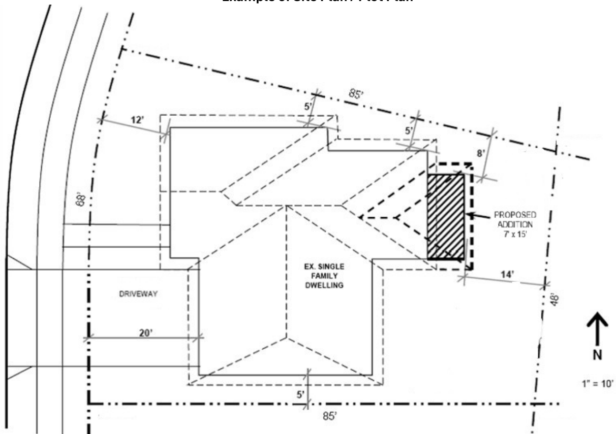
Example of Site Plan / Plot Plan
